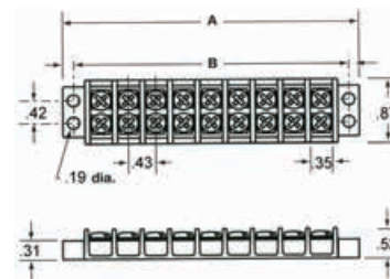
20 AMP
