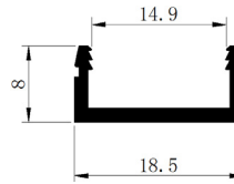
Dimensions (In MM) 120-H3-CHAN-3 (sold separately)
