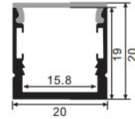
Dimensions (In MM) 120-H3-CHAN2-3 (sold separately)
