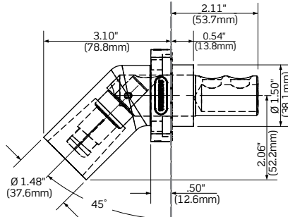
Typical for Double Set Screw Termination
