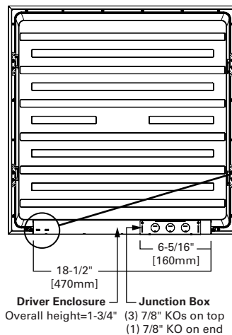
Top View (2' x 2')
