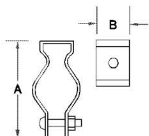
Conduit Hangers STAINLESS STEEL with bolts assembled
