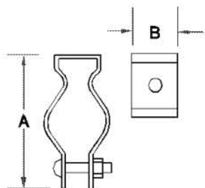
Conduit Hangers WITH BOLT ASSEMBLED ZINC PLATED STEEL AFTER FABRICATION with bolts
