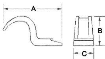
One Hole Strap MALLEABLE IRON
