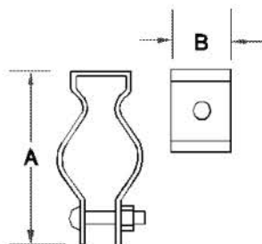
Conduit Hangers WITH BOLT ASSEMBLED ZINC PLATED STEEL AFTER FABRICATION with bolts
