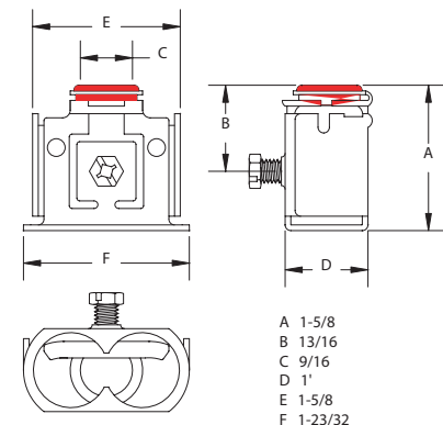
AFC-52 1/2" Duplex Connector
