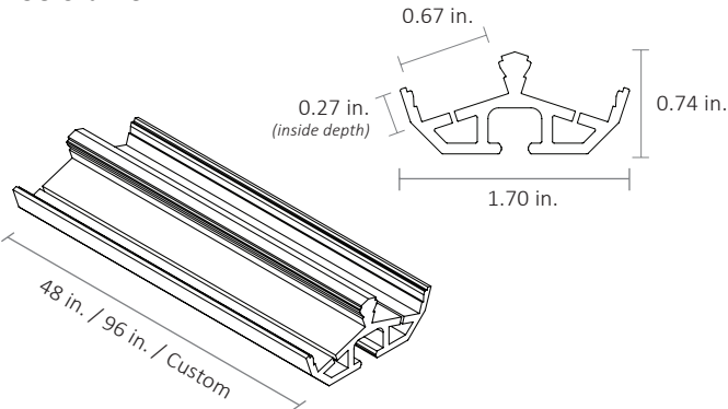
DUO Channel
