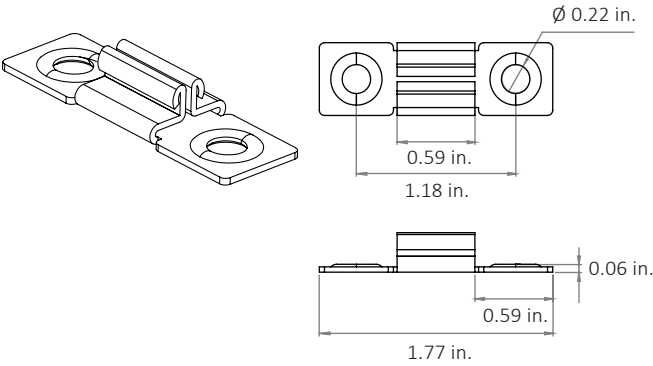
Mounting Clip
