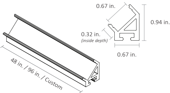
45° Channel
