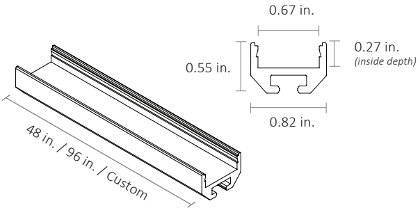
SQUARE Channel
