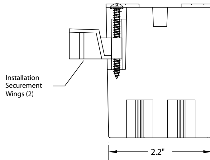
End View
