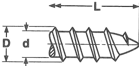
THREADS FOR SELF-TAPPING SCREWS TYPE A
