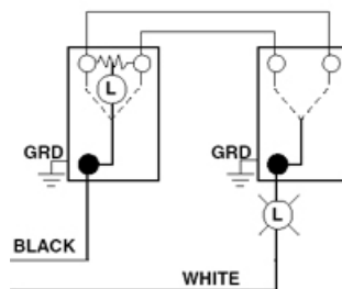
Wiring Diagram 3-Way Lighted
