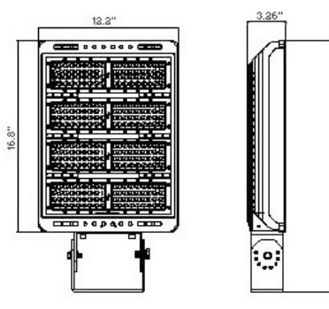
Trunnion
