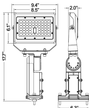
Straight Arm / Slip Fitter Adjustable Combo - 50W
