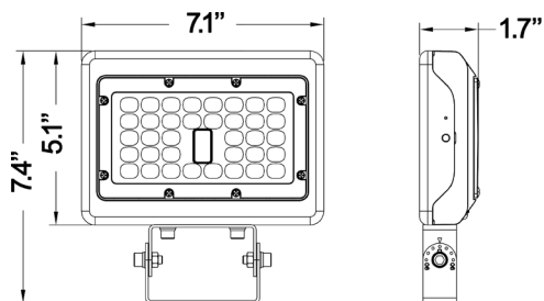
Trunnion Bracket - 15W/ 30W
