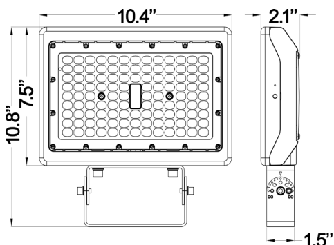
Trunnion Bracket - 80W
