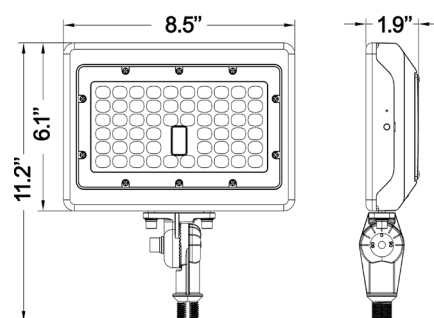
Knuckle Bracket - 50W
