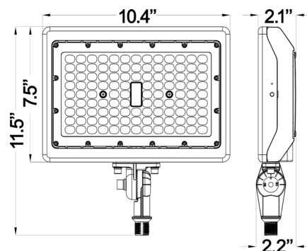
Knuckle Bracket - 80W
