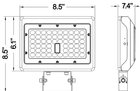
Trunnion Bracket - 50W
