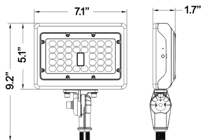
Knuckle Bracket - 15W/30W
