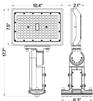
Straight Arm / Slip Fitter Adjustable Combo - 80W
