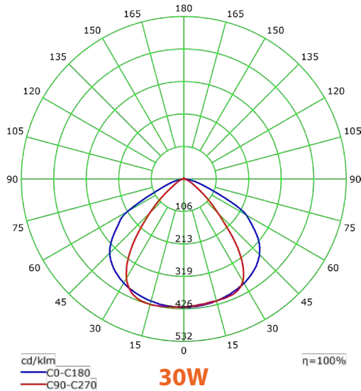
Illuminance at a Distance(Beam Angle)
