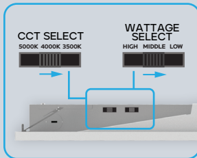
DRIVER WITH CCT & WATTAGE SELECT SWITCH
