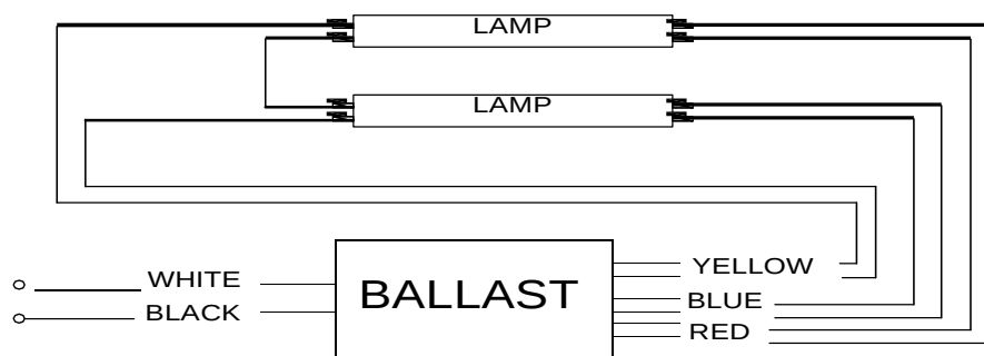
2 Lamps application BALLAST MUST BE GROUNDED
