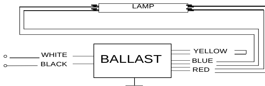
1 Lamp application BALLAST MUST BE GROUNDED YELLOW WIRE MUST BE SHORTED
