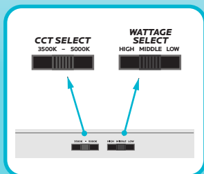
CCT & WATTAGE SELECT SWITCH ON THE SIDE
