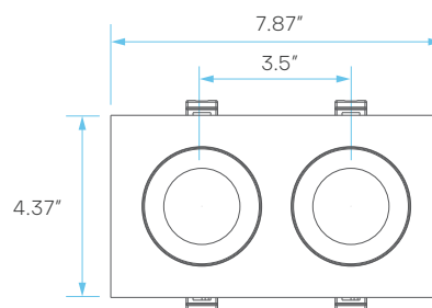
2 HEAD CUTOUT: 7.25" X 3.75"
