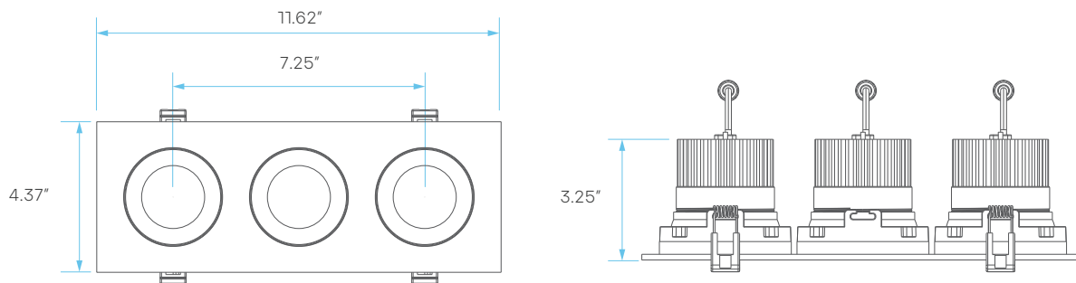
3 HEAD CUTOUT: 10.82" X 3.75"
