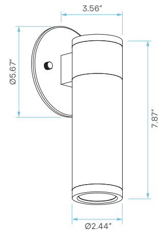
ASSEMBLED VIEW
