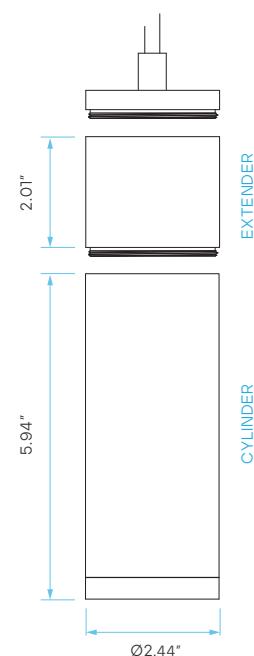
ASSEMBLED VIEW
