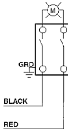
Wiring Diagram Double Pole
