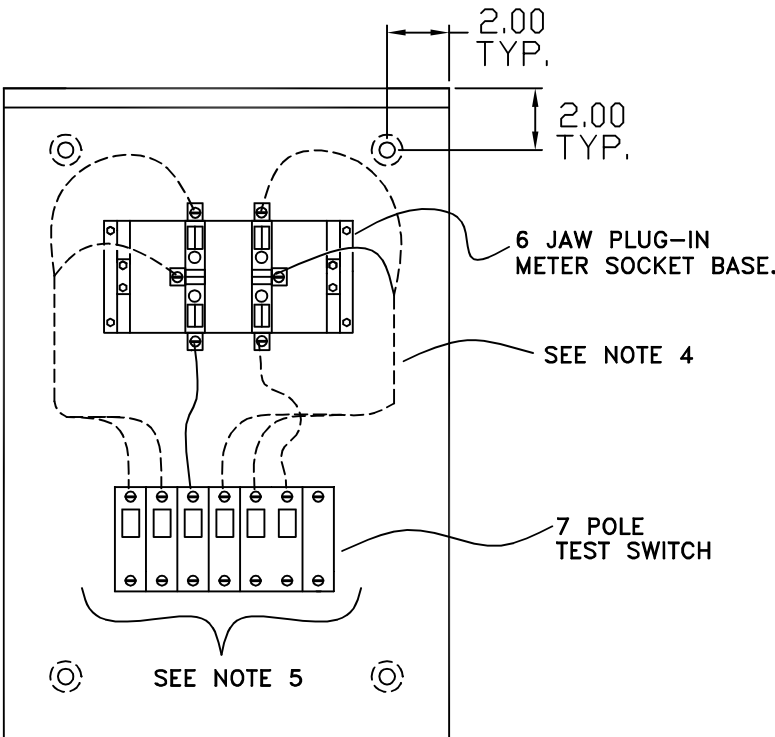
FRONT VIEW – NO COVER FOR MS7P-1L
