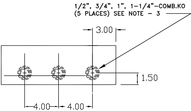
BOTTOM VIEW
