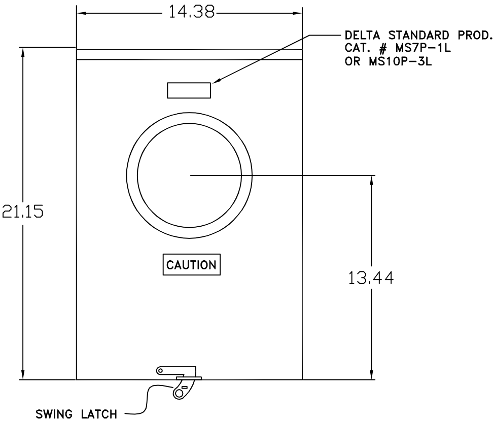
TYPICAL FRONT VIEW
