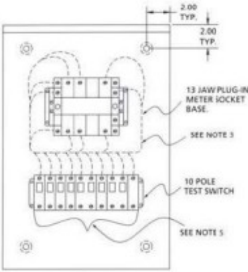
FRONT VIEW NO COVER MS10P-TS
