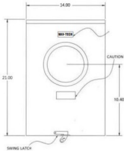
TYPICAL FRONT VIEW
