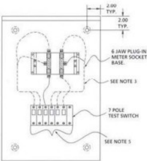
FRONT VIEW NO COVER MS7P-TS
