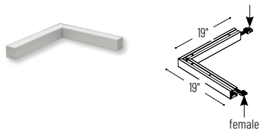
NLIN-L L-Connector
