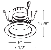
NLPR-5641 5"/6" Reflector
