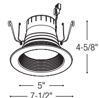
NLPR-5642 5"/6" Baffle
