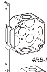
4RB-50-FB
