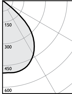
Candela Curve
