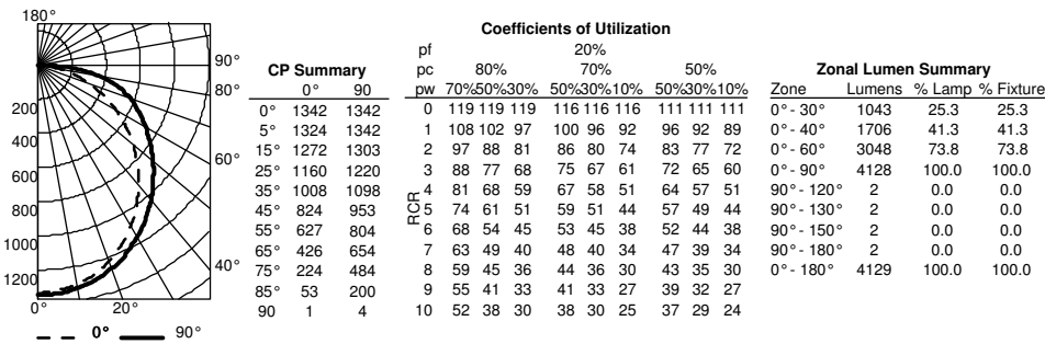
BLC 2X4 4000LM 80CRI 35K ASDM, 4129 Delivered Lumens.
