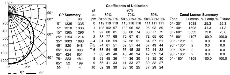
BLC 2X2 4000LM 80CRI 35K ASDM, 4109 Delivered Lumens.
