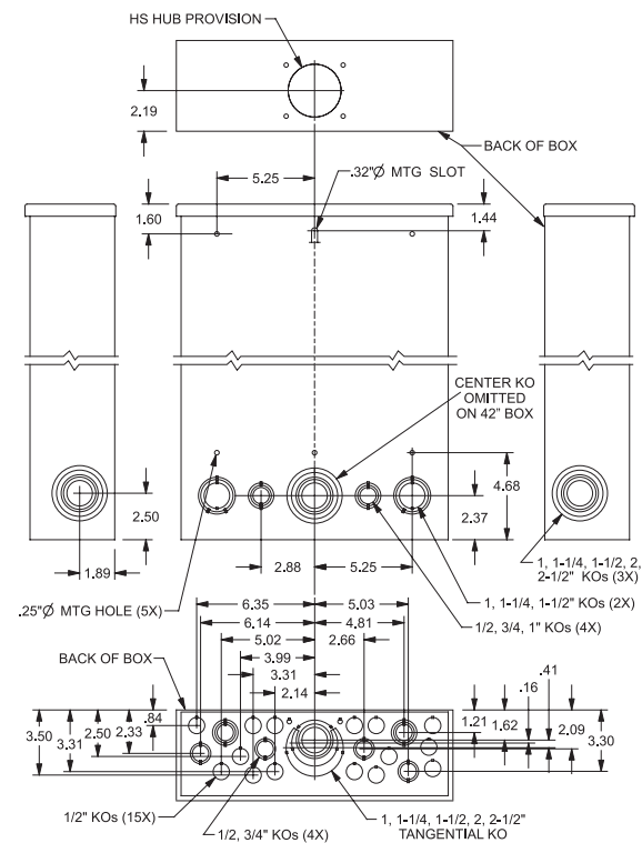
ES, PL, and Generator Ready 1 and 3 Phase Load Centers Outdoor
