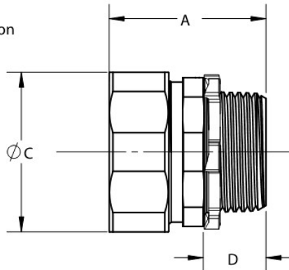
RT Compression Connector
